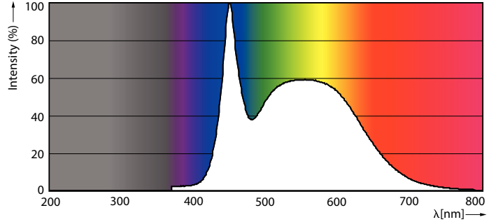
Spectral Power Distribution Colour - EcoHome LEDBulb 10W E27 6500KHV 1PF/20AR
