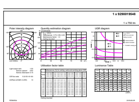
Light Distribution Diagram - EcoHome LEDBulb 10W E27 6500KHV 1PF/20AR
