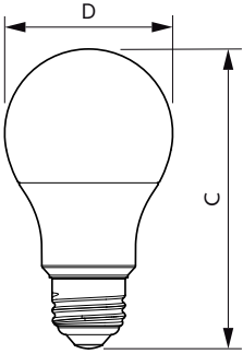
Bulb A60 120V 6-40W 450lm 5000K E26 ND
