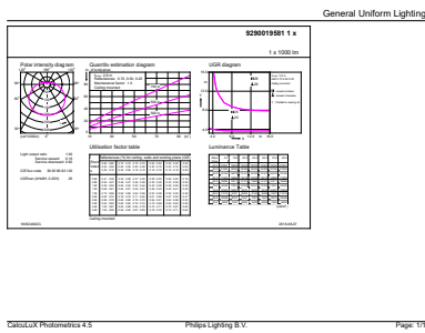
General uniform lighting - 10A19/LED/850/FR/P/ND 4/4FB
