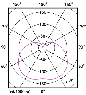
Light Distribution Diagram - 45HB/LED/850/ND FB 6/1
