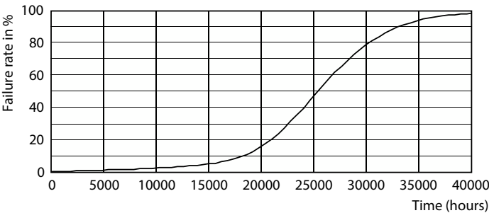
Life Expectancy Diagram - LEDBulb 19W E27 6500K W A25 1PF/6 MX
