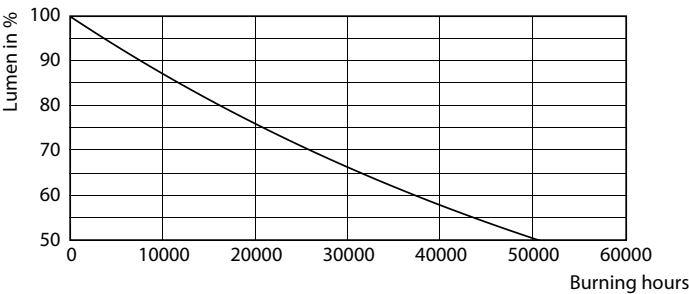
Lumen Maintenance Diagram - LEDBulb 19W E27 6500K W A25 1PF/6 MX
