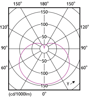
Light Distribution Diagram - LEDBulb 19W E27 6500K W A25 1PF/6 MX
