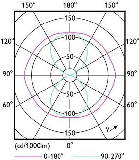
Light Distribution Diagram - TForce LED Road 84-55W E40 730
