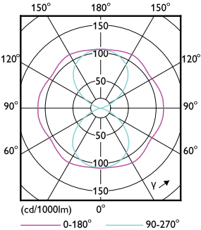
Light Distribution Diagram - TForce LED Road 112-68W E40 730
