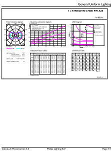
General uniform lighting - CLA LEDBulb DT9-60W E27 CRI90 A60 CL
