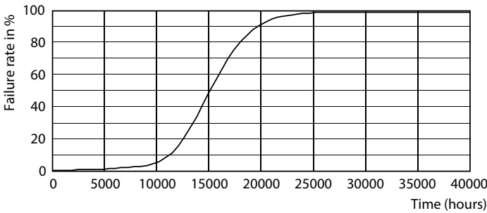
Life Expectancy Diagram - CLA LEDLuster ND 6.5-60W P45 E14 827 CL
