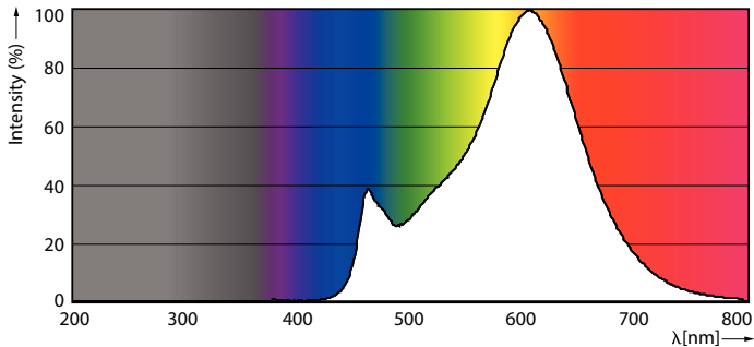
Spectral Power Distribution Colour - CLA LEDLuster ND 6.5-60W P45 E14 827 FR
