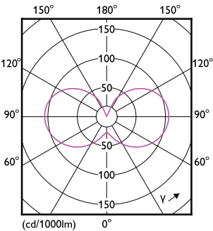
Light Distribution Diagram - CLA LEDLuster ND 6.5-60W P45 E14 840 FR
