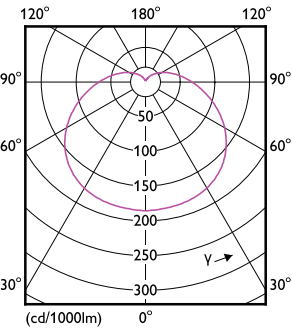
Light Distribution Diagram - CorePro LEDbulb ND 17-120WA67E27 827FR
