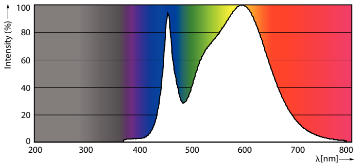
Spectral Power Distribution Colour - CorePro LEDbulb ND 15.5-120WA67E27 840FR
