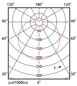
Light Distribution Diagram - LED 200W A110 E27 CDL 230V FR ND 1PF/6
