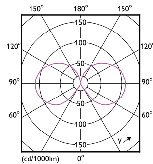
Light Distribution Diagram - CLA LEDBulb ND 17-150W A67 E27 827 CL
