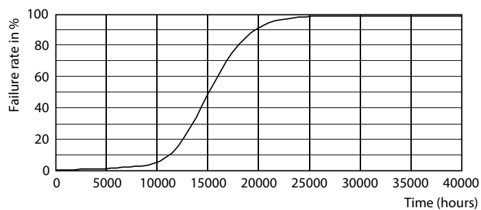
Life Expectancy Diagram - CorePro LEDbulb D 5-40W A60 E27 927
