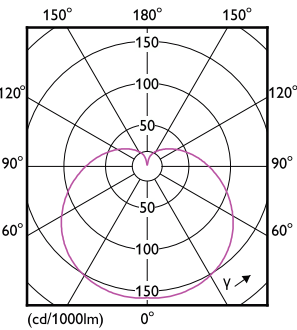
Light Distribution Diagram - CorePro LEDbulb D 8.5-60W A60 E27 927
