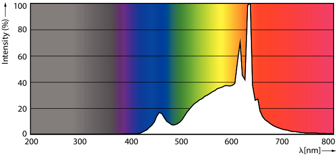
Spectral Power Distribution Colour - CorePro LEDbulb D 13-100W A60 E27 927
