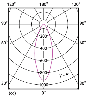
Light Distribution Diagram - 7PAR20/COR/827/F40/DIM/120V B 6/1FB
