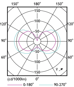
Light Distribution Diagram - LED diamond_giant 35W E27 CL DIM
