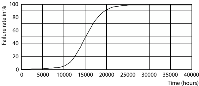
Life Expectancy Diagram - LED diamond_giant 35W E27 CL DIM
