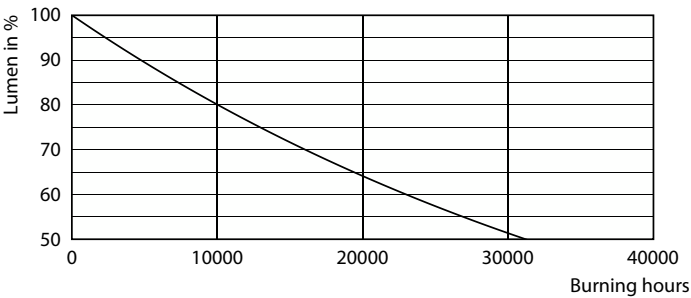
Lumen Maintenance Diagram - LED diamond_giant 35W E27 CL DIM
