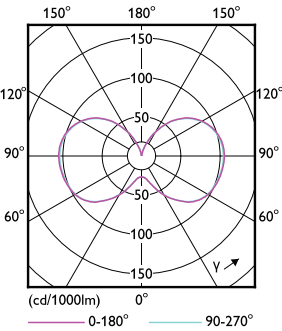
Light Distribution Diagram - 36CC/LED/830/ND E26 BB 12/1
