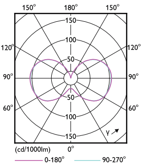
Light Distribution Diagram - 36CC/LED/840/ND EX39 BB 12/1
