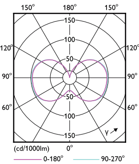
Light Distribution Diagram - 100CC/LED/850/ND EX39 BB 6/1
