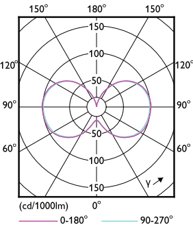
Light Distribution Diagram - 120CC/LED/840/ND EX39 BB 6/1
