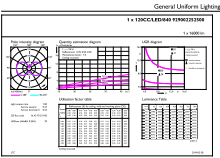
Light Distribution Diagram - 120CC/LED/840/ND EX39 BB 6/1
