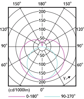
Light Distribution Diagram - 14T5HE/COR/46-840/MF21/G 25/1
