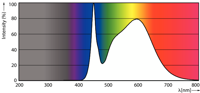
Spectral Power Distribution Colour - 14T5HE/COR/46-840/MF21/G 25/1
