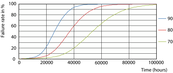
Life Expectancy Diagram - 14T5HE/COR/46-850/MF21/G 25/1
