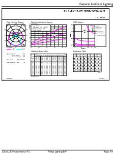
General uniform lighting - 14.5T8/COR/48-840/MF21/G/DIM 25/1
