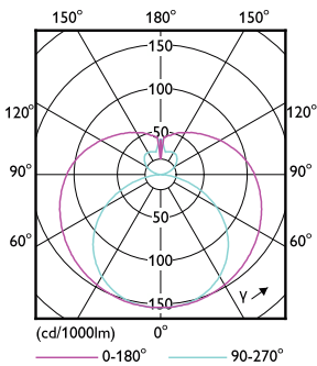
Light Distribution Diagram - 14.5T8/COR/48-840/MF21/G/DIM 25/1
